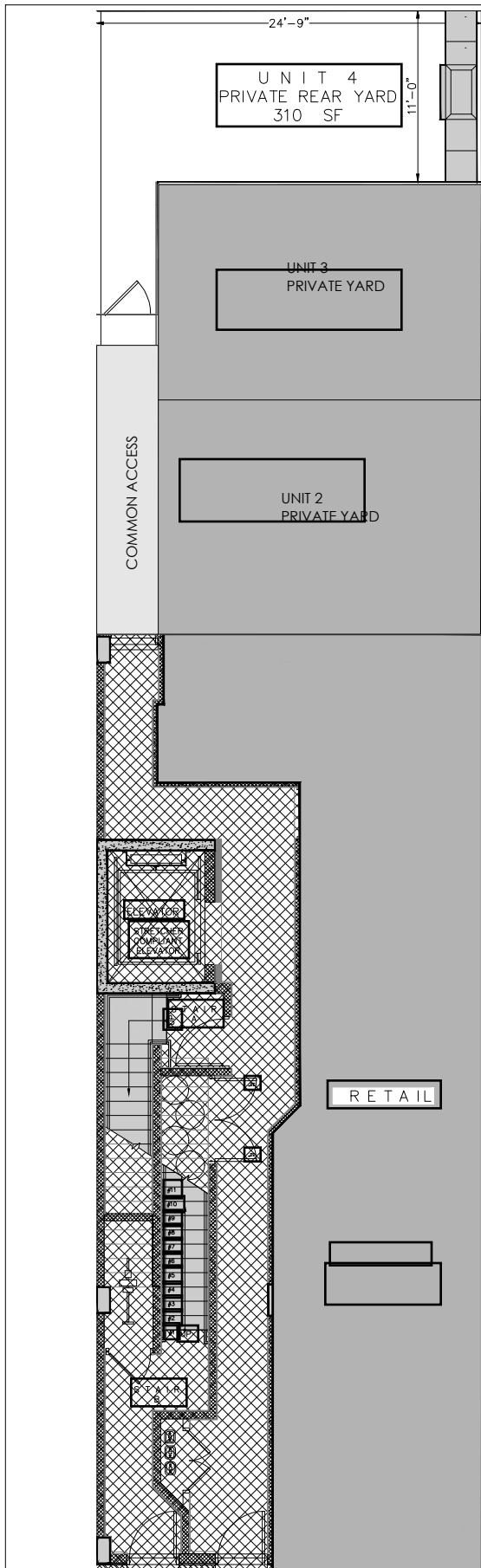
FIRST FLOOR: REAR YARD : UNIT 4
