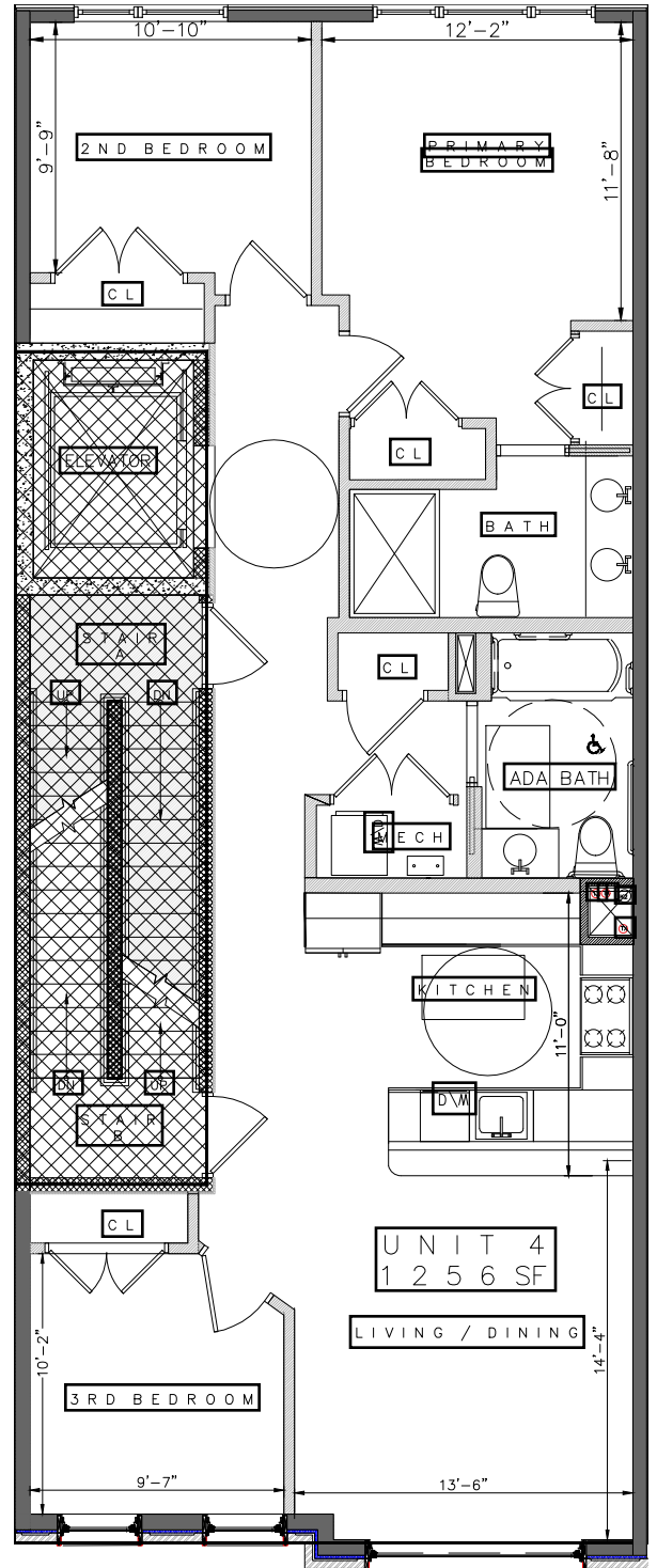
FOURTH FLOOR: UNIT 4
