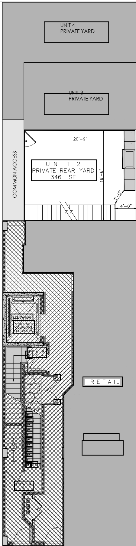
FIRST FLOOR: REAR YARD : UNIT 2 SCALE: 3/32"=1'-0"
