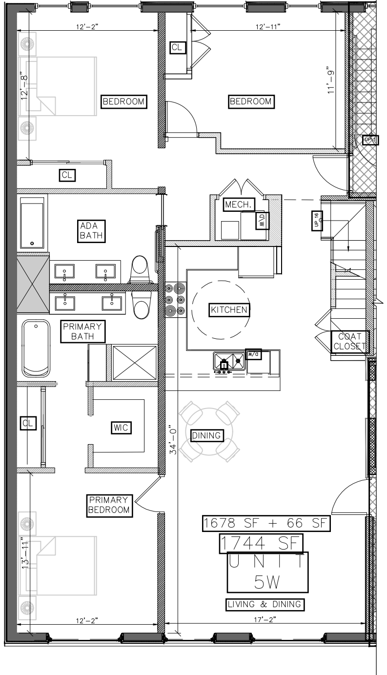
FIFTH FLOOR: UNIT 5W SCALE: 1/8"=1'-0"
