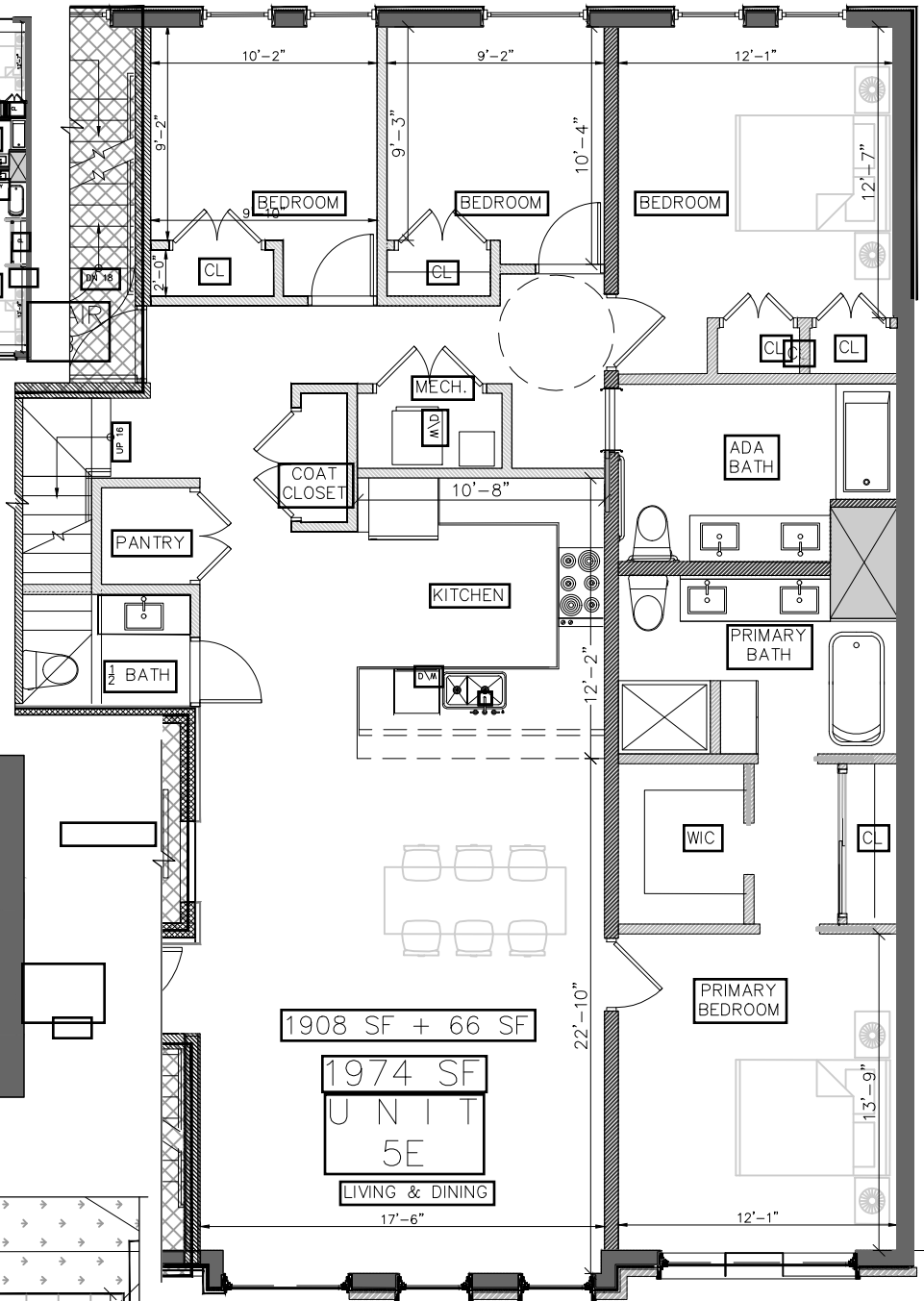
FIFTH FLOOR: UNIT 5E SCALE: 1/8"=1'-0"
