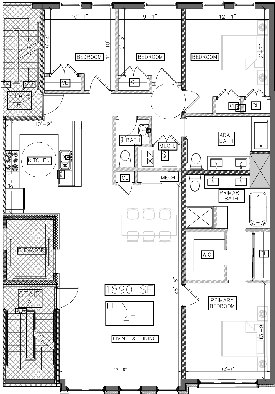
FOURTH FLOOR: UNIT 4E SCALE: 1/8"=1'-0"
