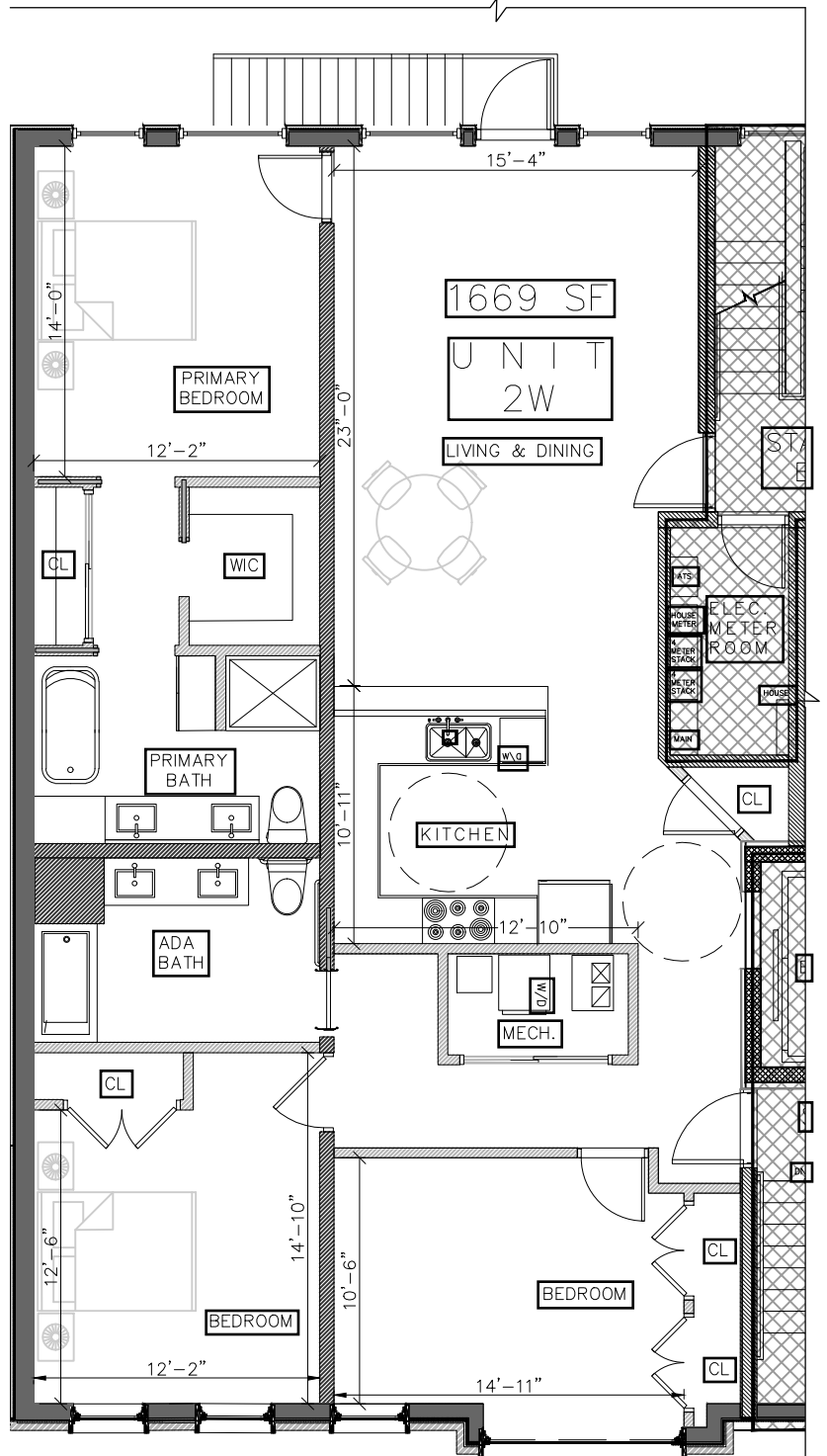
SECOND FLOOR: UNIT 2W SCALE: 1/8"=1'-0"
